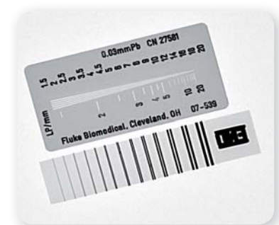
BoltX – 6.6 lp/mm image
